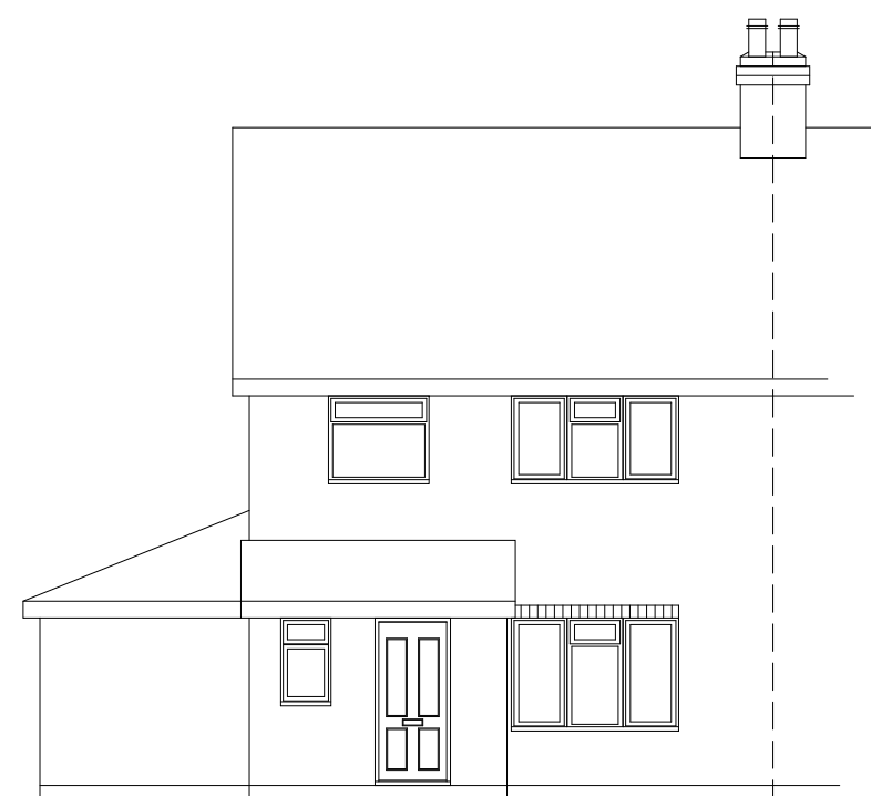
Proposed Front
